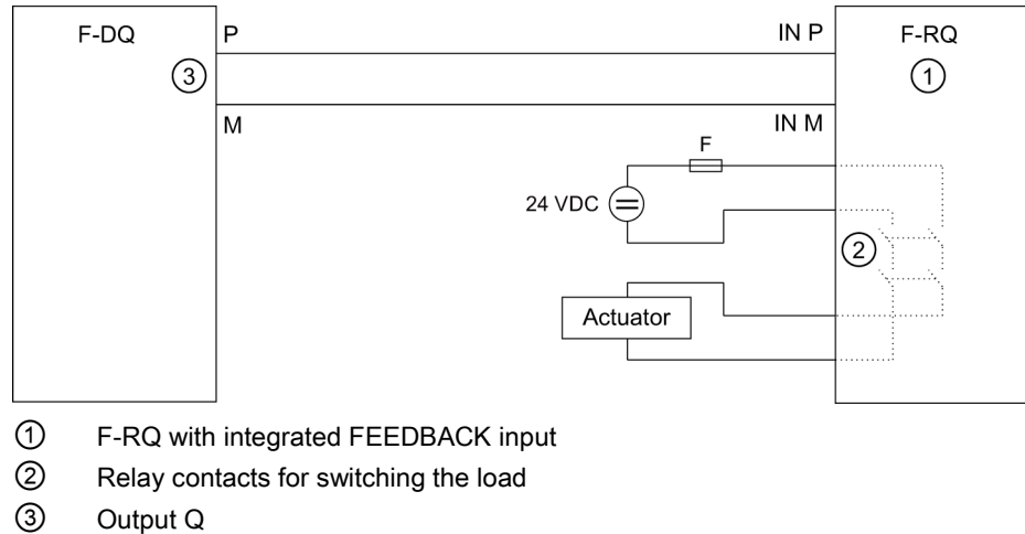
Figure 5-6 Wiring example for the FDBACK instruction
