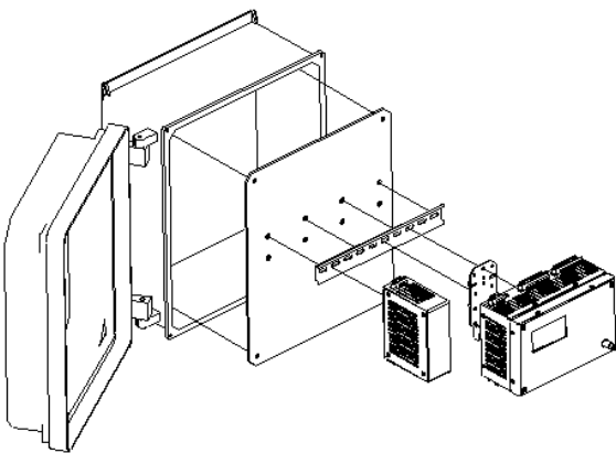
Figure 4: 1900/55 Replacement Kit
