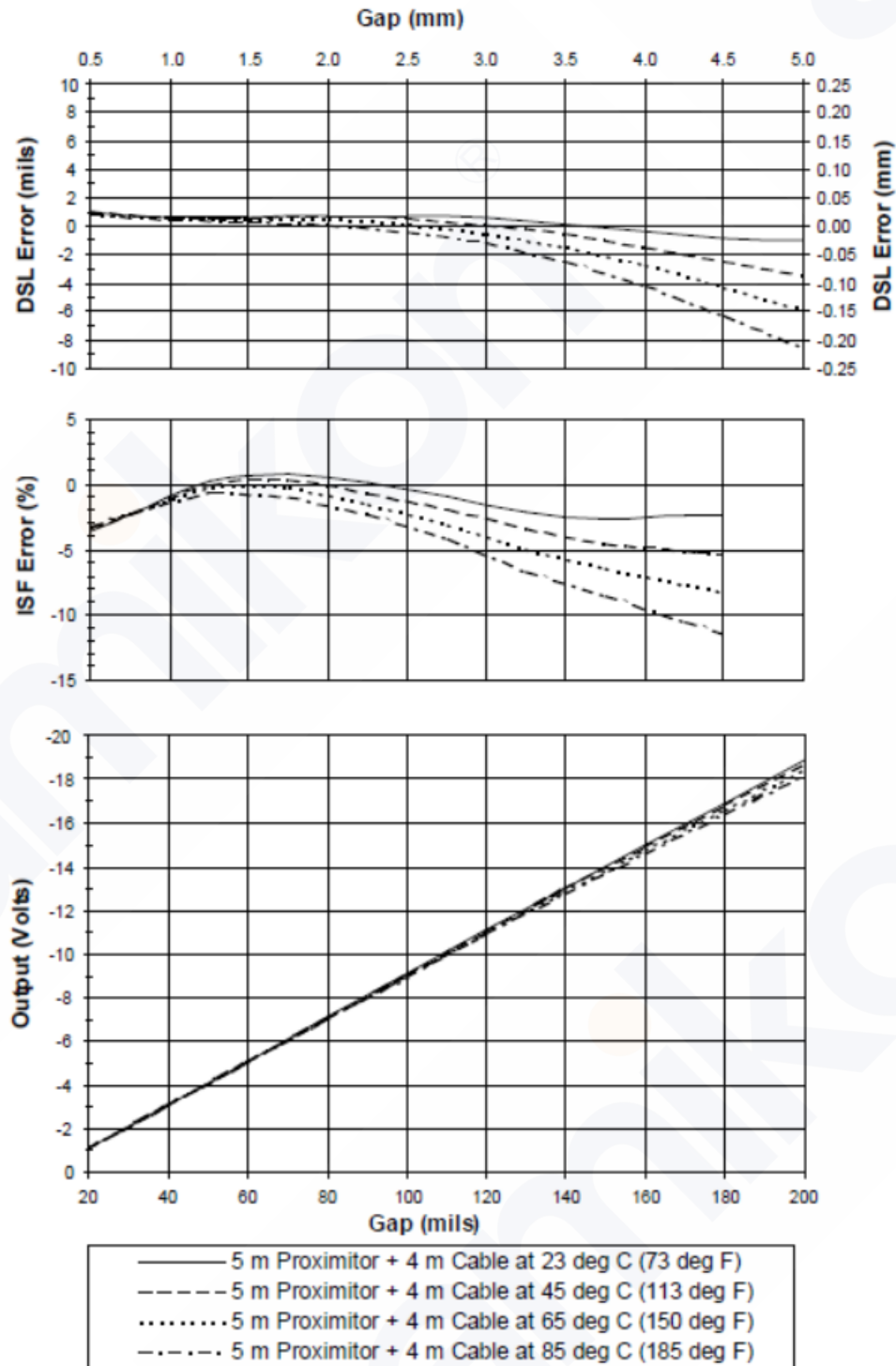
Figure 6: Typical 3300 XL 11 mm 5 m Proximitor Sensor with 4 m Extension Cable @ High Temperature
