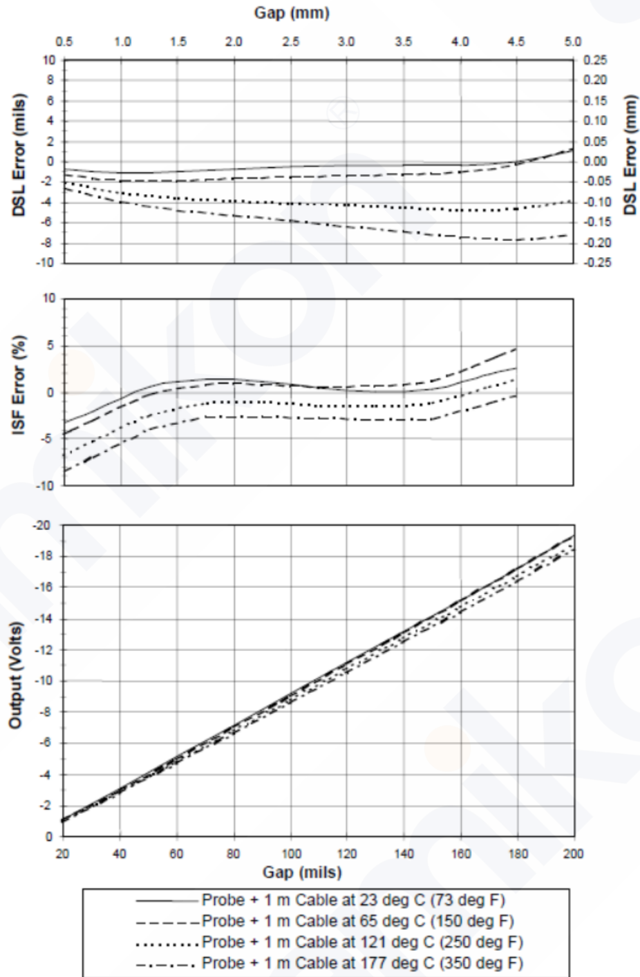
Figure 4: Typical 3300 XL 11 mm Probe + 1m Cable @ High Temperature (Proximitor Sensor + 4m of Extension Cable @ 25 °C)
