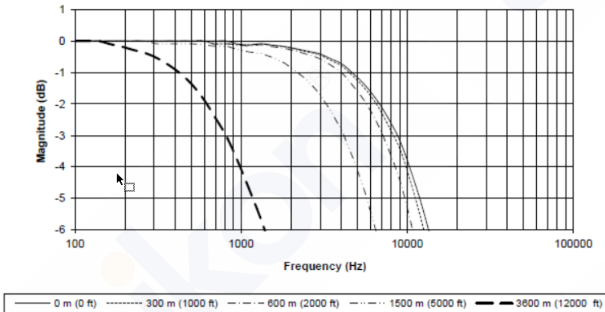
Figure 9: Frequency Response, magnitude of typical 3300 XL 11mm System
