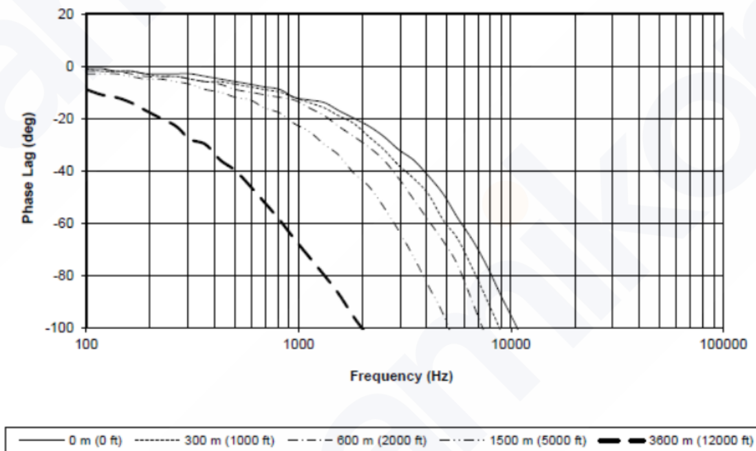
Figure 10: Frequency Response, phase change of typical 3300 XL 11mm System
