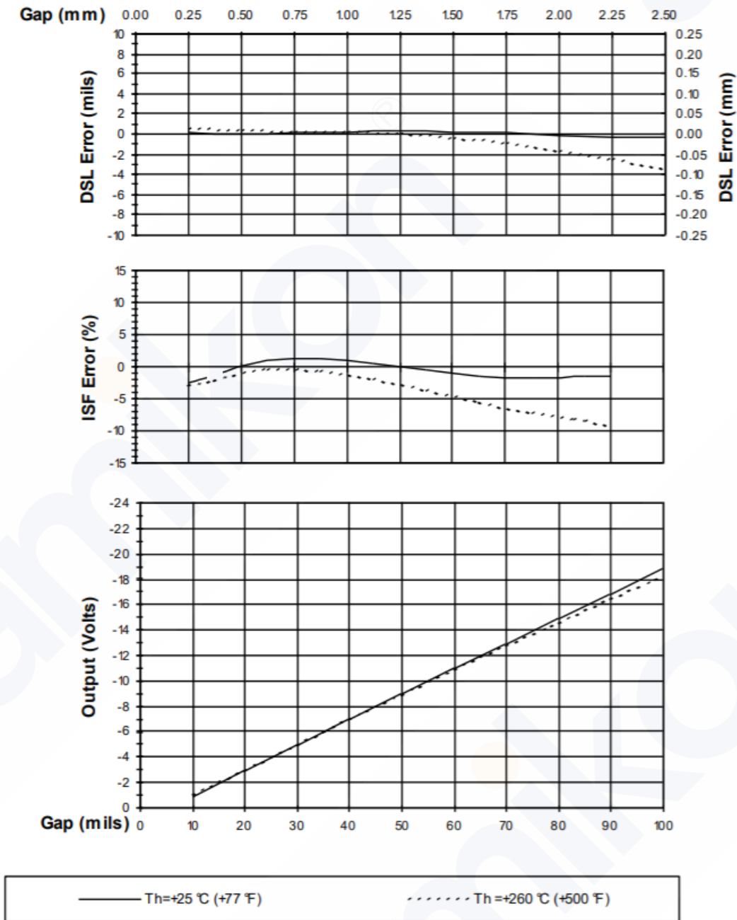
Figure 8: Typical 3300 XL Extended Temperature Range Probe and 4 m Extended Temperature Range Extension Cable at T_h (Proximitors Sensor and Probe Tip with 1-foot Cable are at +25\text{ }^{\circ}\text{C} )
