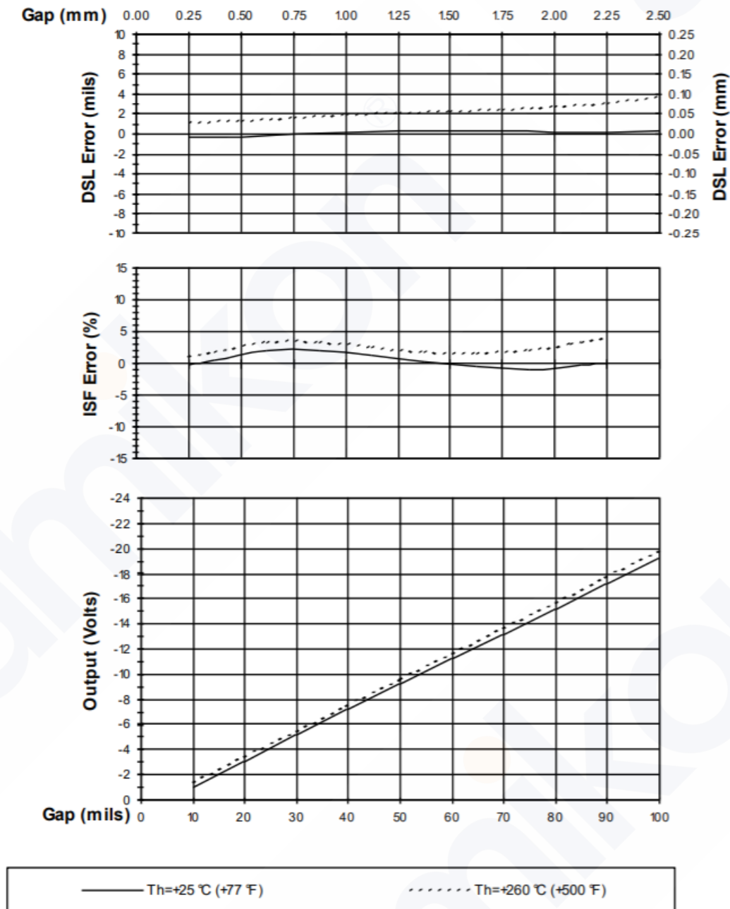
Figure 9: Typical 3300 XL Extended Temperature Range Probe and 8 m Extended Temperature Range Extension Cable at T_h (Proximitor Sensor and Probe Tip with 1-foot Cable are at +25\text{ }^{\circ}\text{C} )
