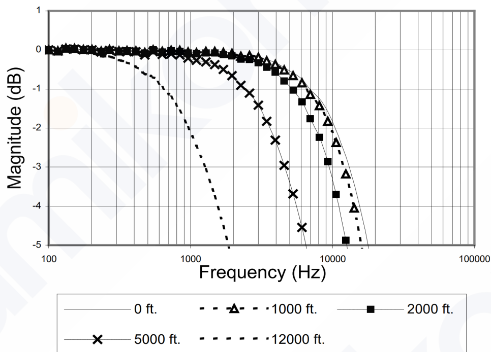
Figure 1: Frequency Response with Different Field Wiring Lengths without Barriers (1 m System)
