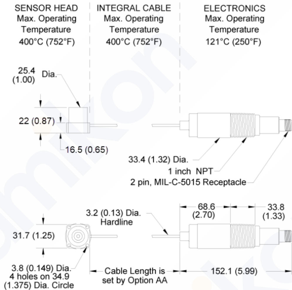
Figure 1: 330750 System Dimensional Drawing
