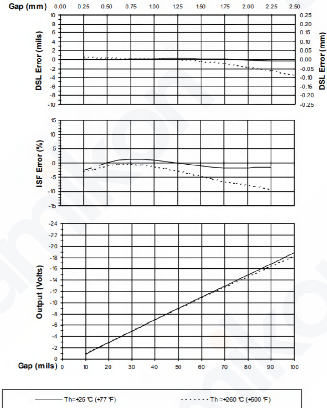
Figure 8: Typical 3300 XL Extended Temperature Range Probe and 4 m Extended Temperature Range Extension Cable at T_h (Proximator Sensor and Probe Tip with 1-foot Cable are at +25^{\circ}\text{C} )
