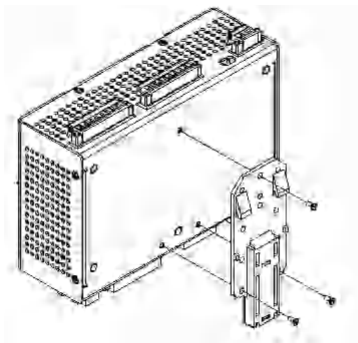
Figure 1: DIN Rail Mount
