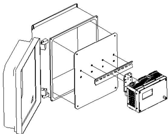
Figure 3: NEMA 4X/IP66_WP_Housing
