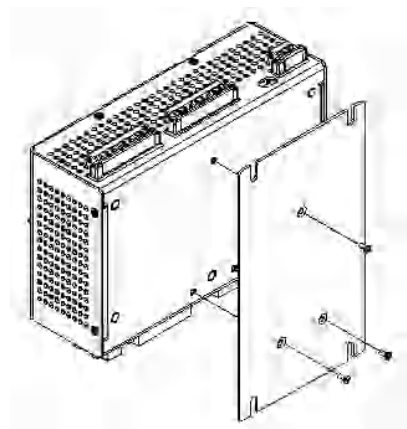
Figure 2: Bulkhead Mount
