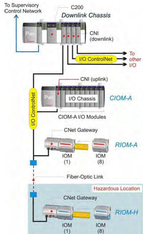
Figure 10-1 I/O Control Network Overview
