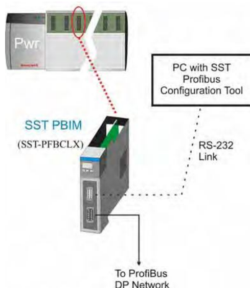
Figure 9-1 PROFIBUS Interface Module
