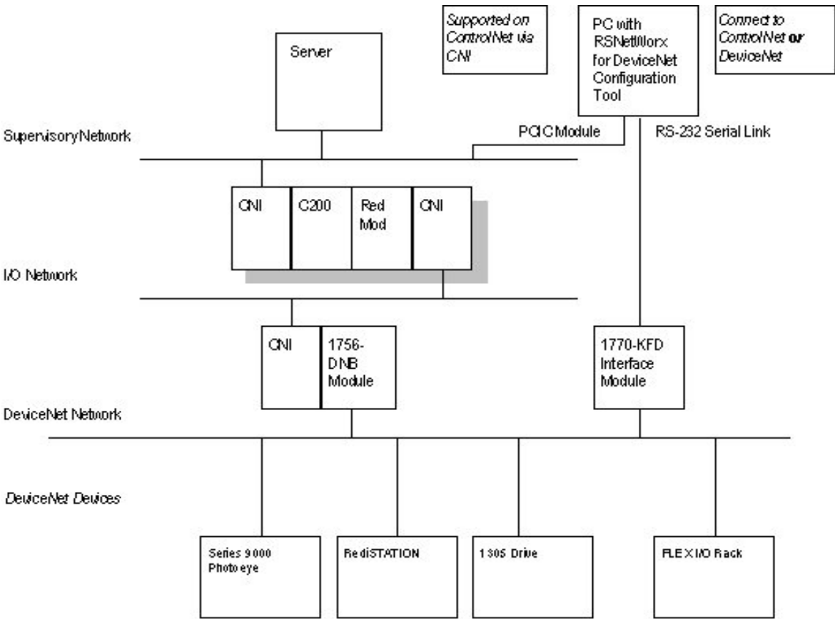
Figure 8-1 Redundant Controller Experion platform with DeviceNet Interface
