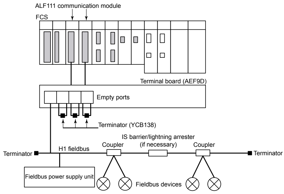
Figure Dual-redundant System Configuration
