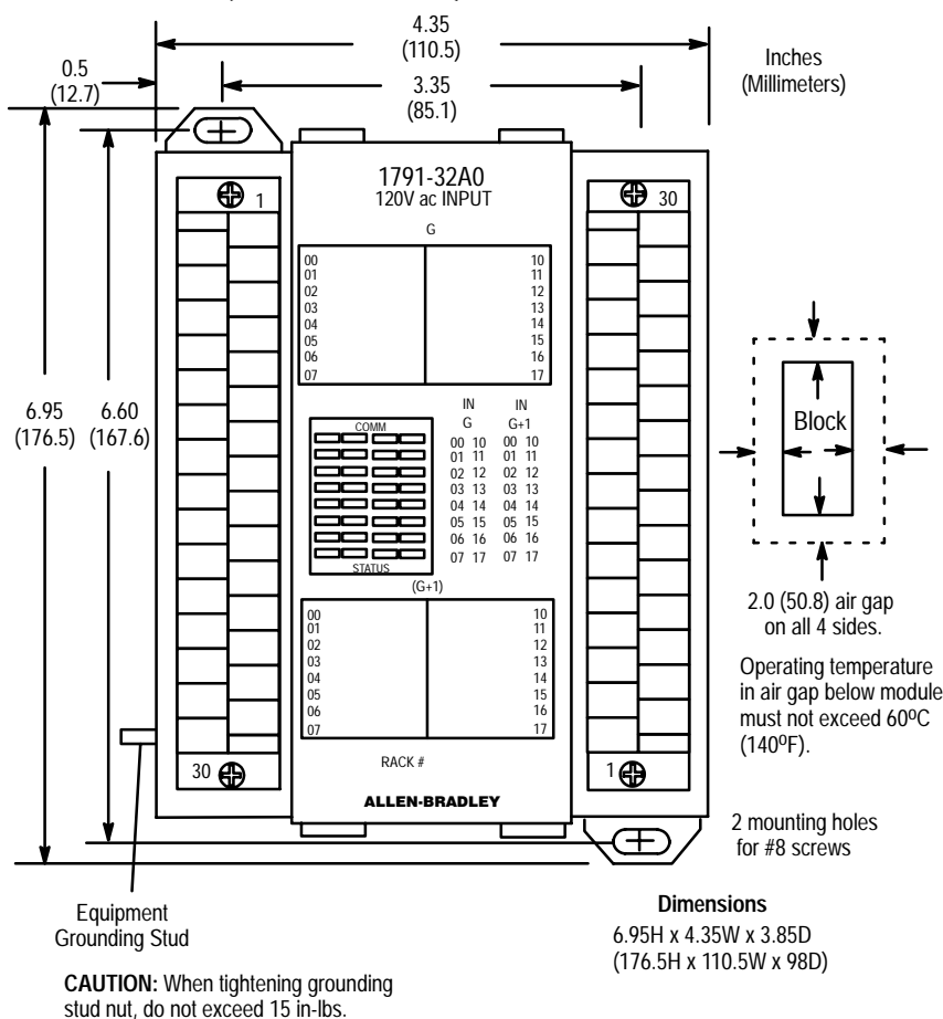
Figure 1 Mounting Dimensions for the Block I/O Module Cat. No. 1791-32A0 (PLC version shown)
