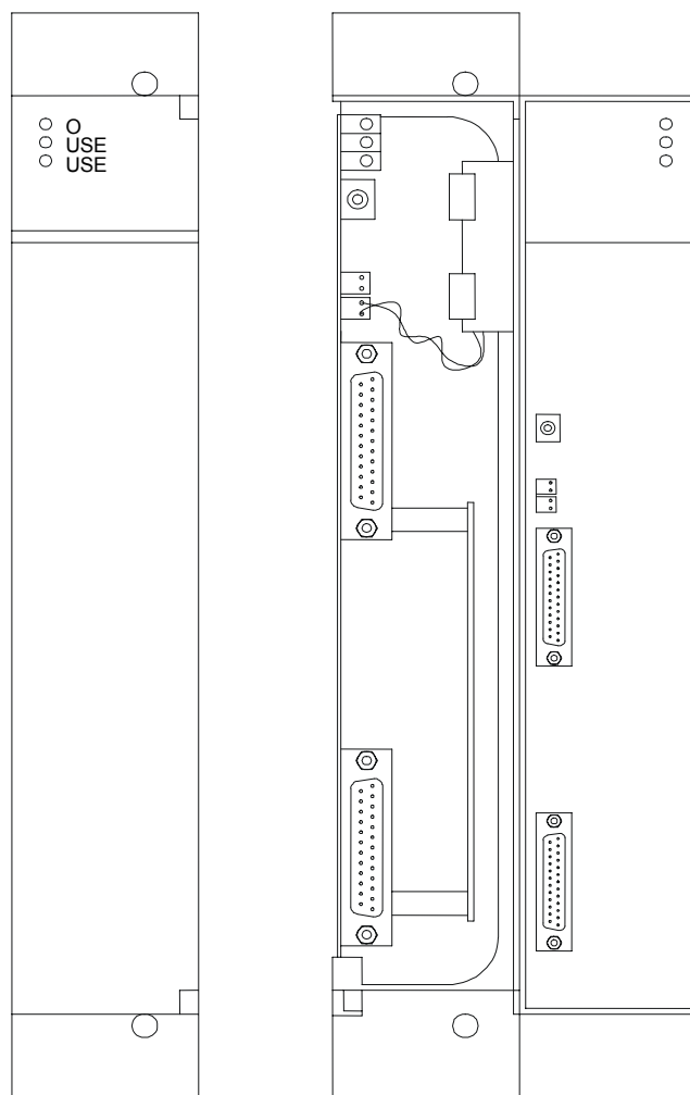
Figure 1.2 - RTM705 Module
