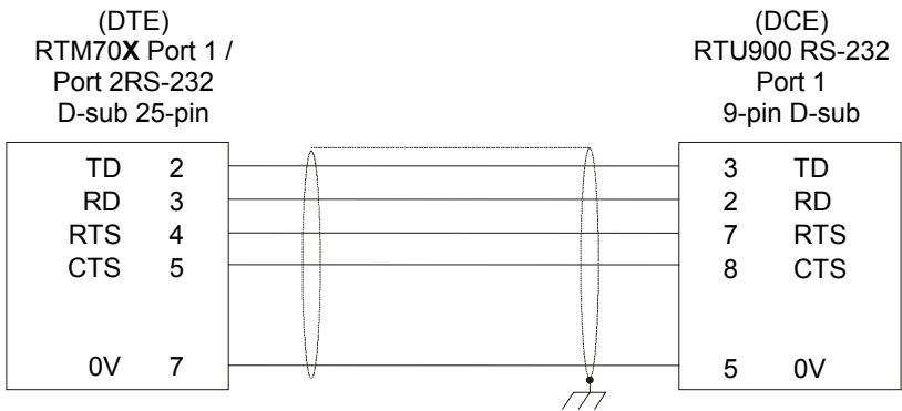
Figure 2.6 - RTM700/705 RS-232 to RTU900 RS-232 (Port 1) Wiring
