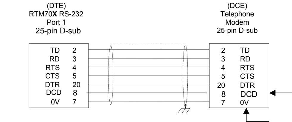
Figure 2.5 - RTM700/705 RS-232 to Telephone Modem Wiring
