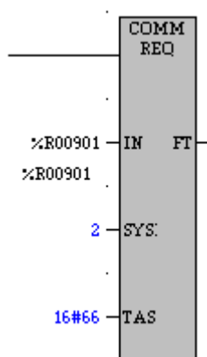
Figure 3.1 – COM_REQ Function
