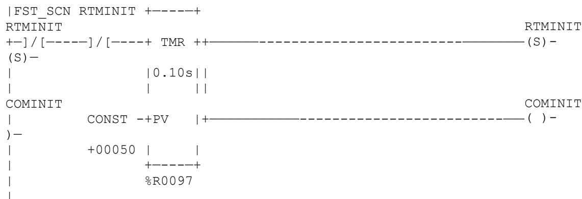
Figure 4.7 – COM_REQ Data Block Ladder Logic Example
