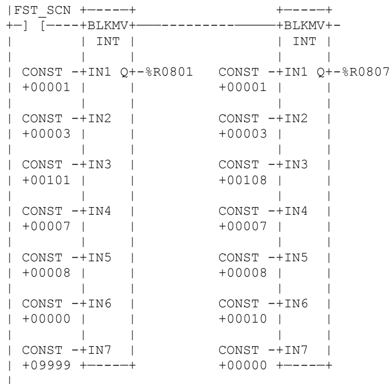
Figure 4.4 – MCB Ladder Logic Example
