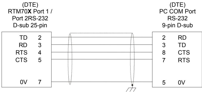
Figure 2.7 - RTM700/705 RS-232 to PC COM Port Wiring
