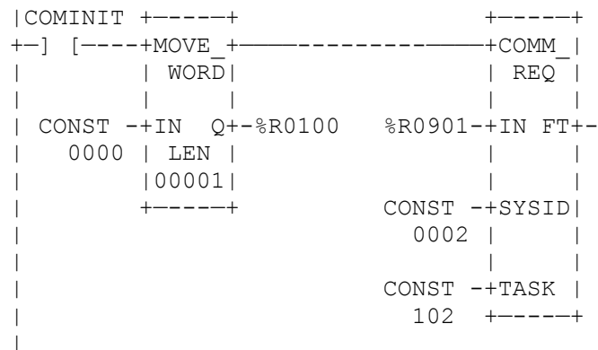
Figure 4.8 – COM REQ Execution Ladder Logic Example
