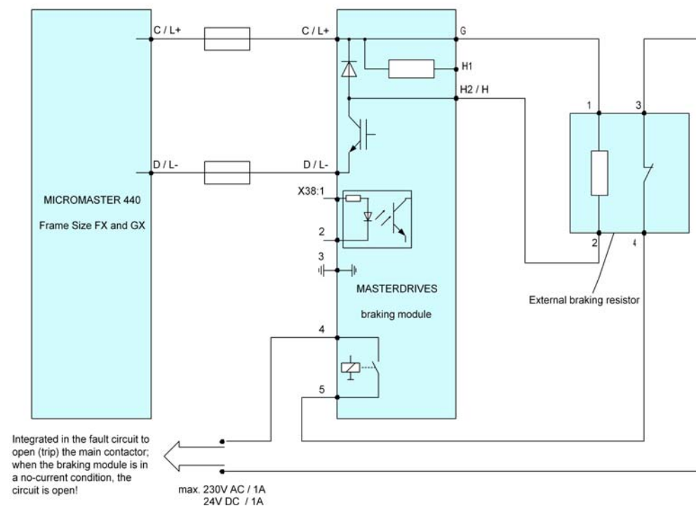
Figure 3-1 Connecting the braking module to drive inverters MM440, FX and GX
