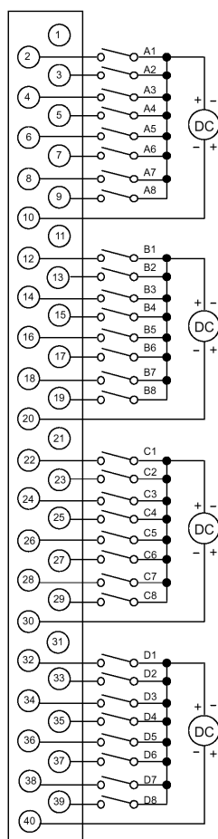
Figure 2. Field Wiring Connections for IC697MDL654
