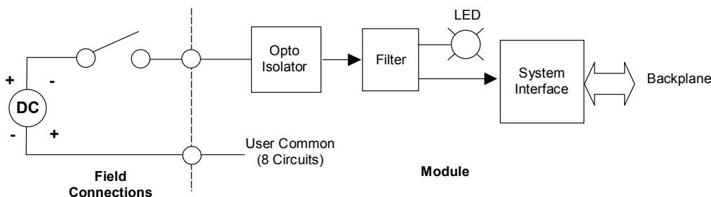
Figure 1. Block Diagram for IC697MDL654
