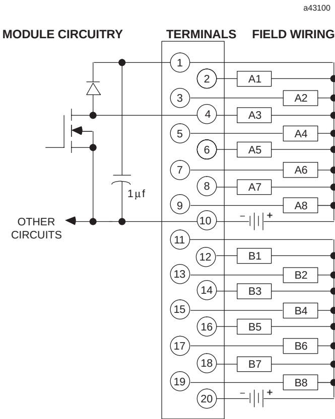
Figure 7-24. IC693MDL741 Output Module Field Wiring
