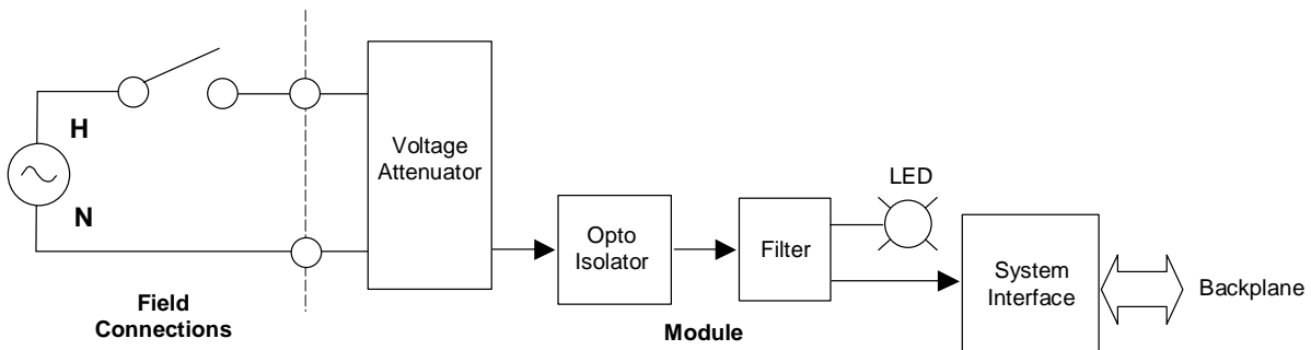
Block Diagram for IC697MDL241
