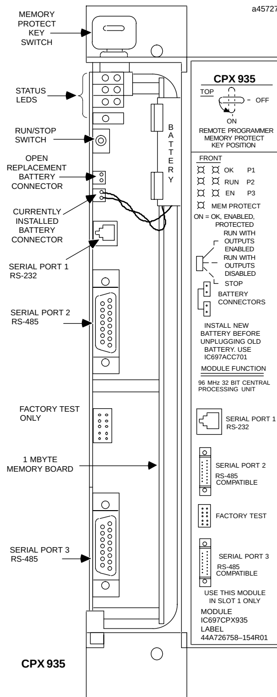
Figure 2. CPX 935 - Location of Major Features
