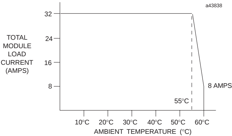
Figure 7-29. Load Current vs. Temperature for IC693MDL930
