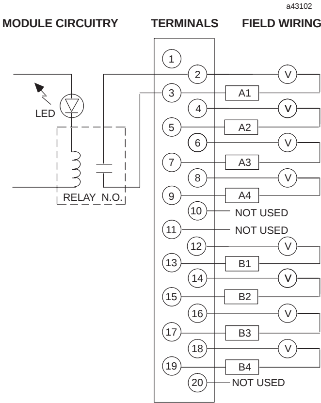
Figure 7-28. IC693MDL930 Output Module Field Wiring
