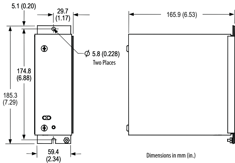
Figure 3 - Mechanical Dimensions
