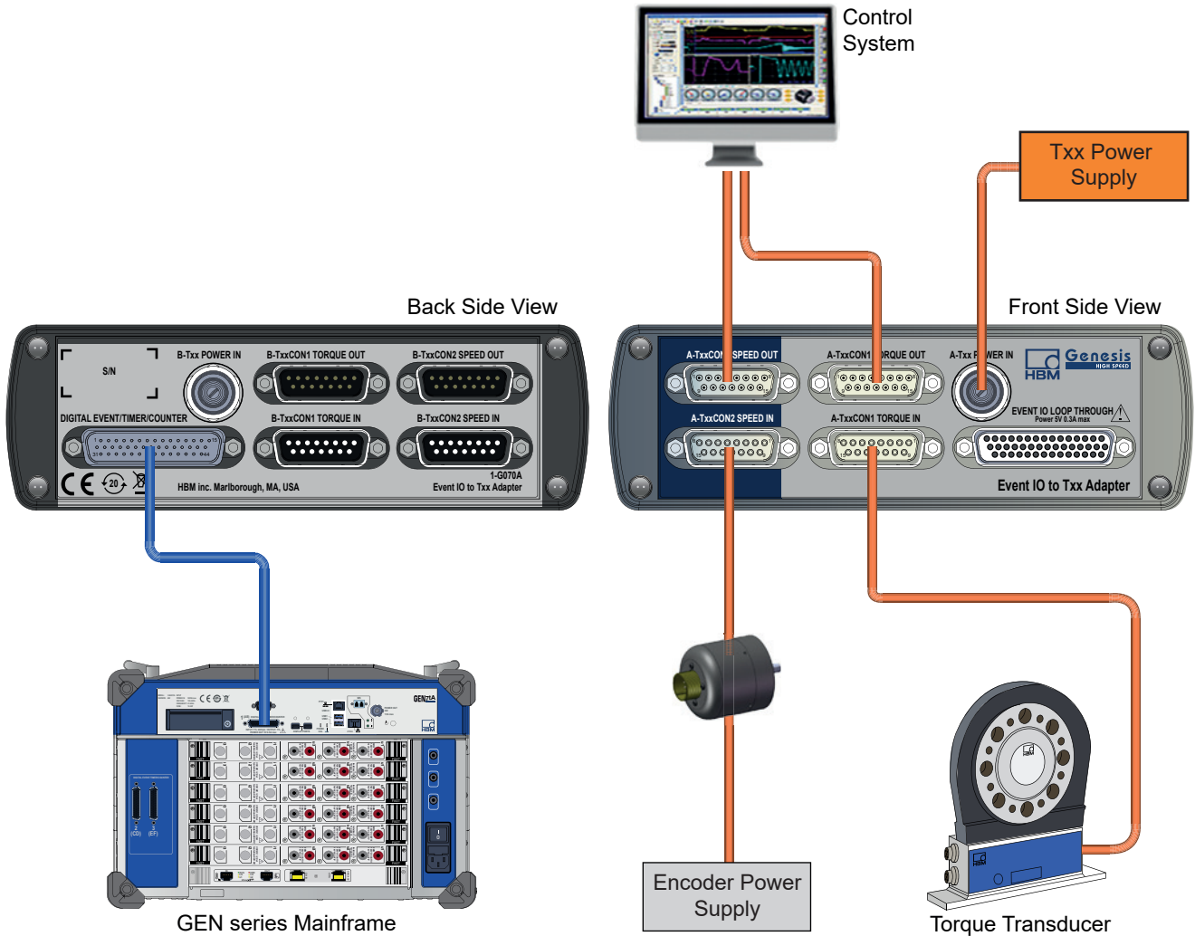
Figure 12: Torque transducer and speed encoder connected to GEN DAQ and control system
