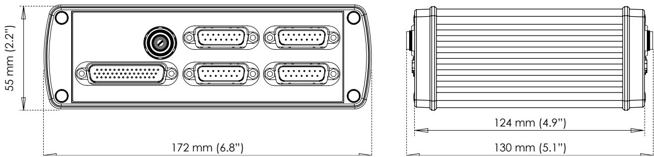
Figure 13: G070A dimensions
