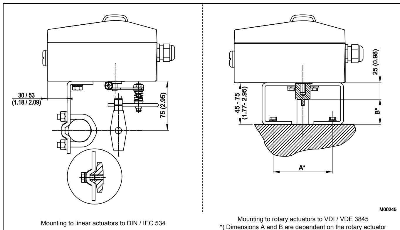
Fig. 14: Mounting drawings
