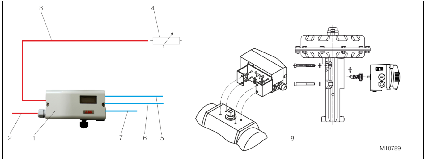
Fig. 10: TZIDC for remote sensors
