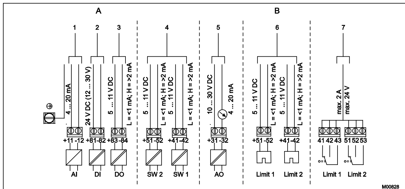
Fig. 8: Pin configuration
