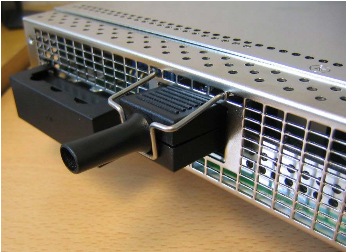
Figure 3 AC Power Connectors and Retaining Clips
