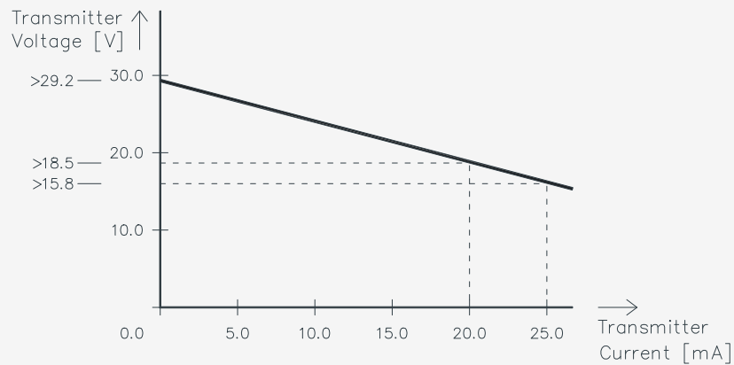
Figure 15-76: Transmitter voltage for passive transmitters
