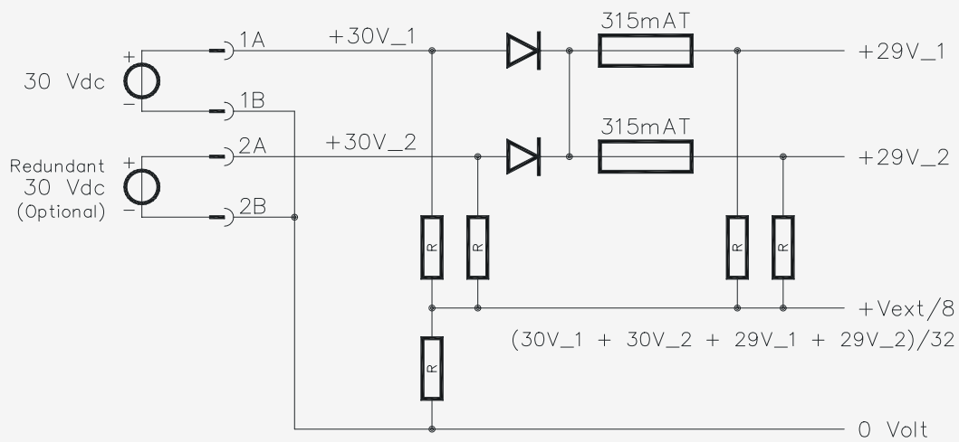
Figure 15-77: Schematic diagram for power distribution with monitoring
