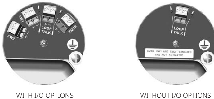
Figure 27. Terminal Box
