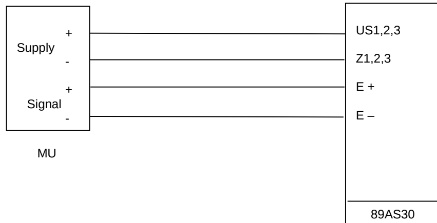
Connection of four-core transducers Possible only if their current consumption < 25 mA
