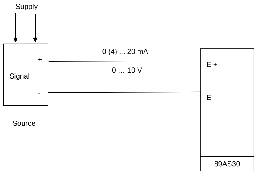
Connection of twin – core transducers
