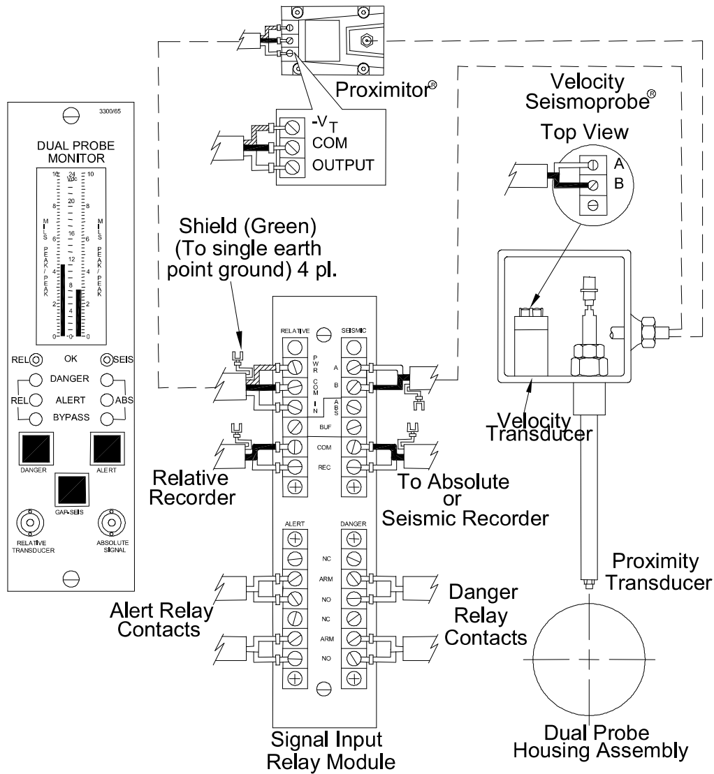
Field wiring diagram for 3300/65 Dual Probe Monitor
