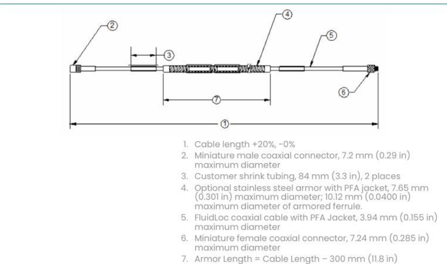
Figure 12: 330877, 3300 XL 50 mm Extension Cable
