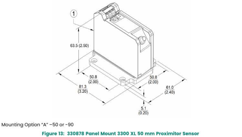
Figure 13: 330878 Panel Mount 3300 XL 50 mm Proximity Sensor
