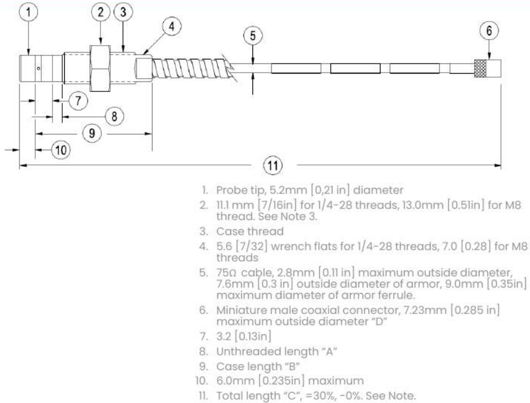
Figure 3: 3300 5mm Proximity Probes, Standard Mount3
