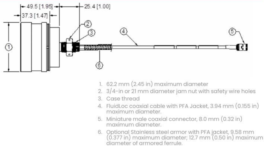
Figure 10: 330876, 3300 XL 50 mm Proximity Probe, Straight Exit
