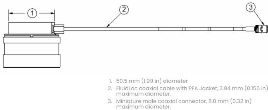
Figure 11: 330876, 3300 XL 50 mm Proximity Probe, Smooth 1.99 Inch Dia. Side Exit Case
