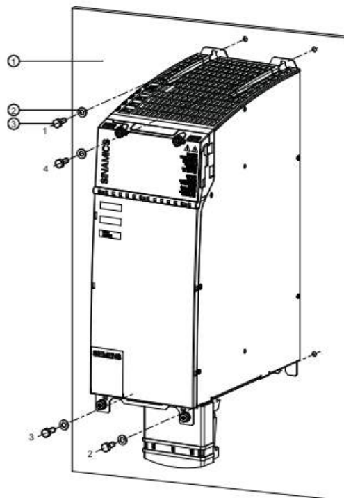
Figure 5-7 Installing an Active Line Module (example, 36 kW)
