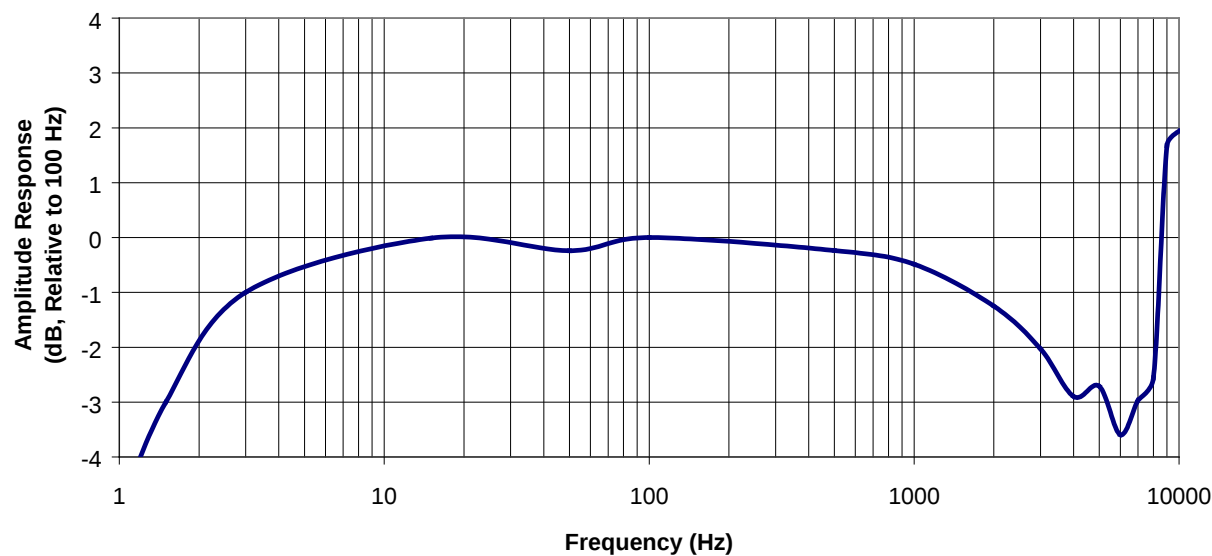
Figure 3: Typical Amplitude Response
