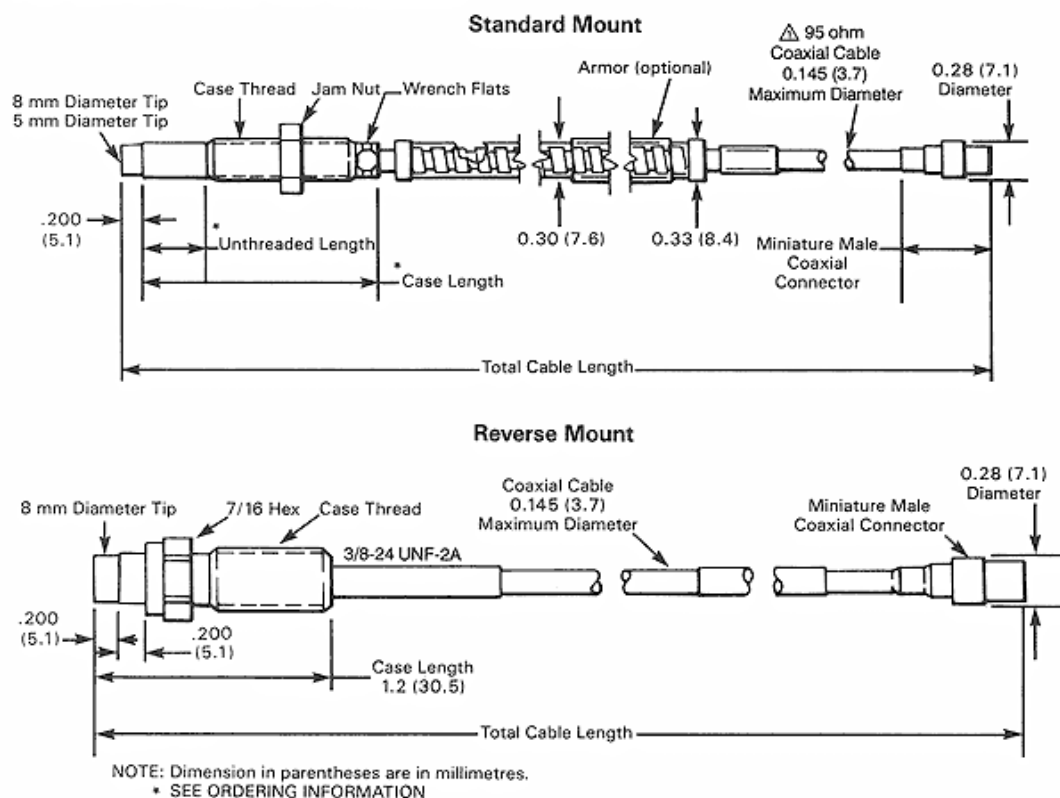
FIGURE 1 \Delta Maximum diameter for 21500 and 21501 probes is 0.111 in. (3.4 mm).
