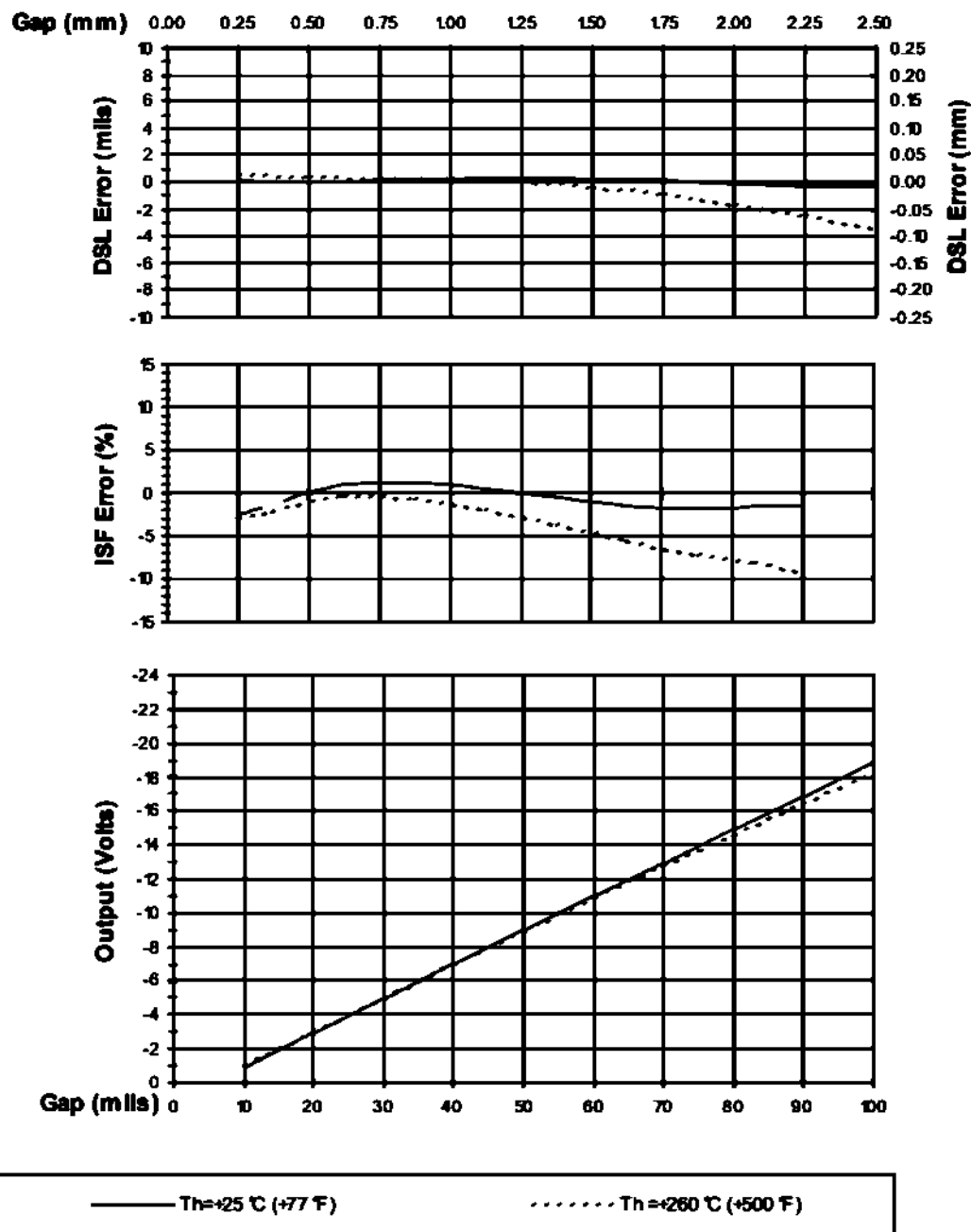
Figure 8: Typical 3300 XL Extended Temperature Range Probe and 4 m Extended Temperature Range Extension Cable at T_h (Proximator Sensor and Probe Tip with 1-foot Cable are at +25^{\circ}\text{C} )
