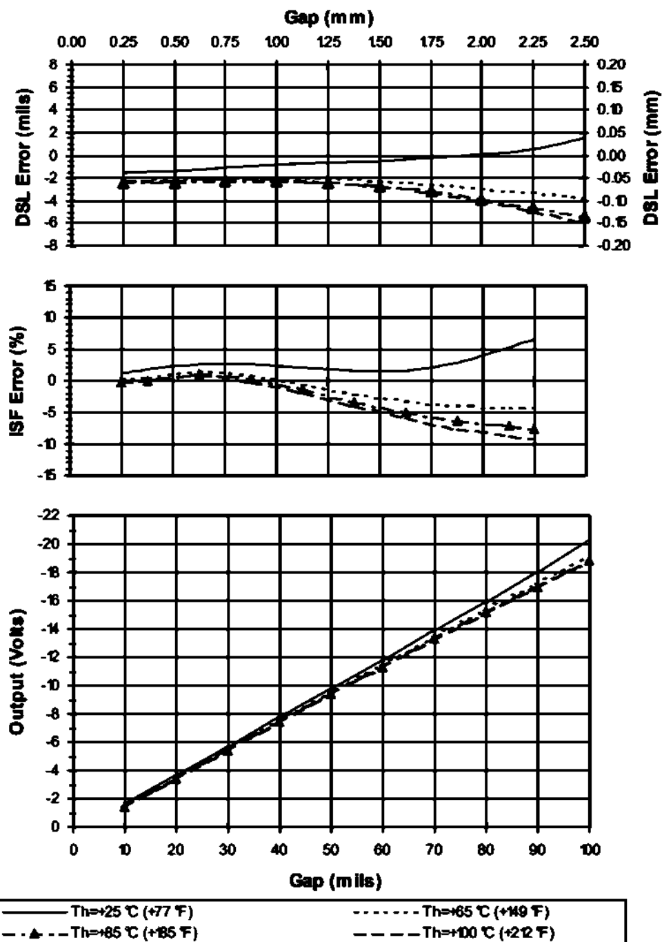
Figure 7: Typical 3300 XL 8 mm 9 m Proximity Sensor with 8 m Extension Cable at T_h (Probe is at 25^\circ\text{C} )
