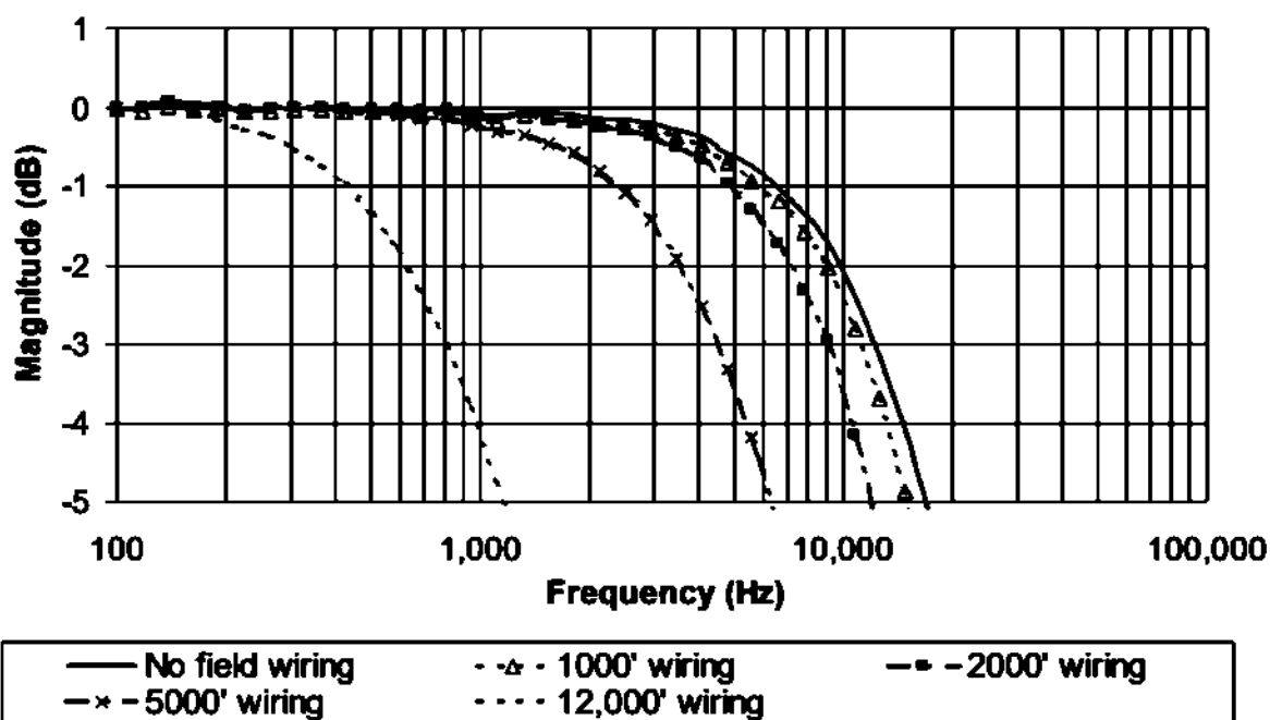
Figure 10: Frequency Response, Typical 3300 XL 8 mm 5 m or 1 m System with Varying Lengths of Field Wiring Attached, No Barriers
