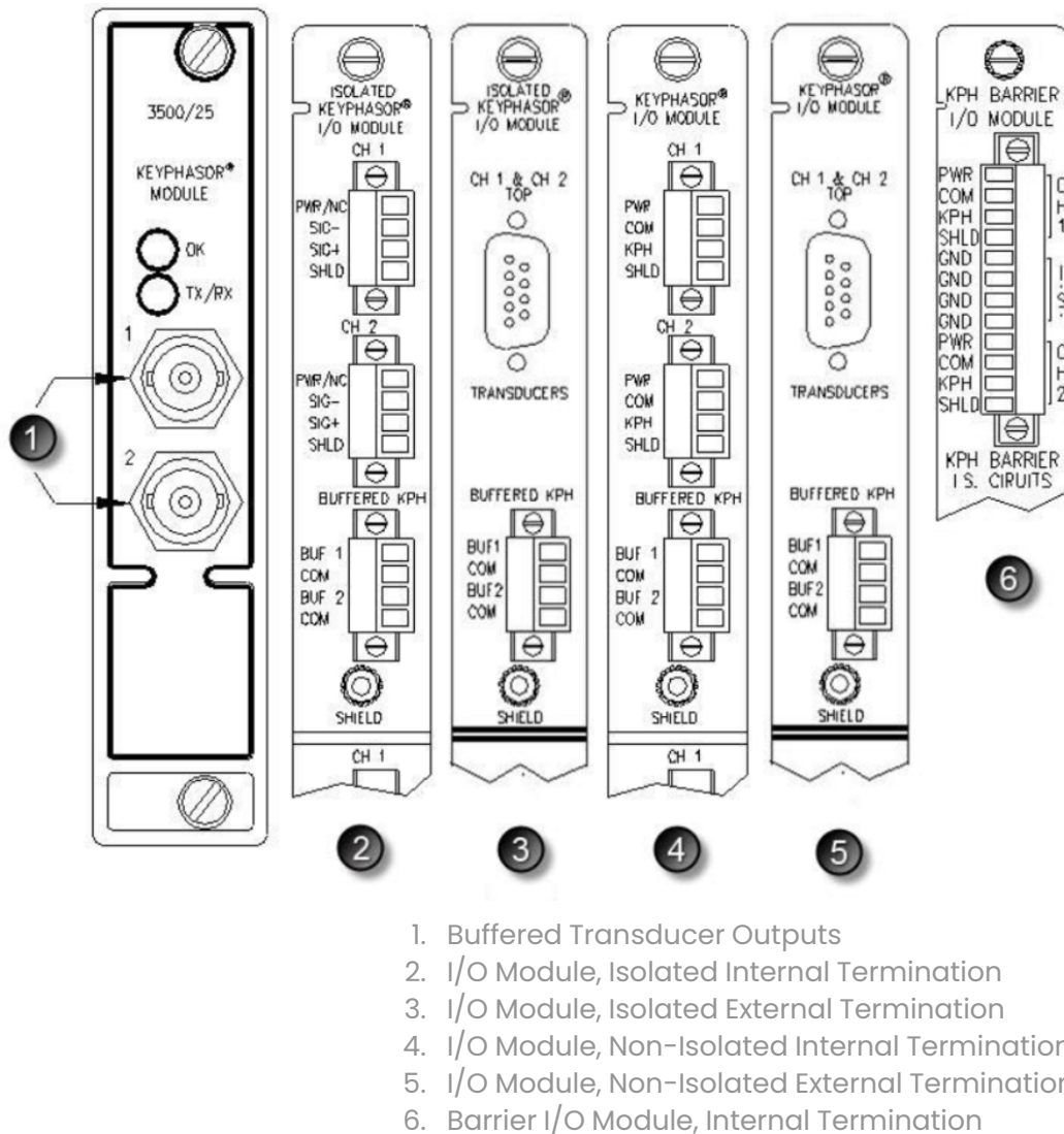
Figure 2: Front and Rear View of 3500/25 Keyphasor module
