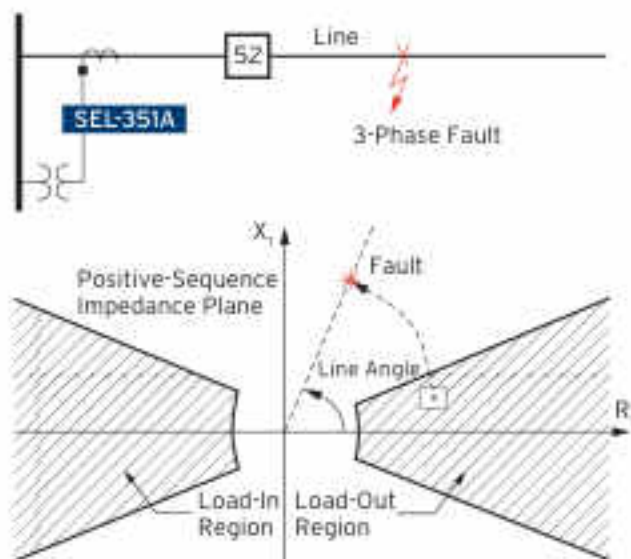
SEL-351A impedance plane showing a fault condition.
