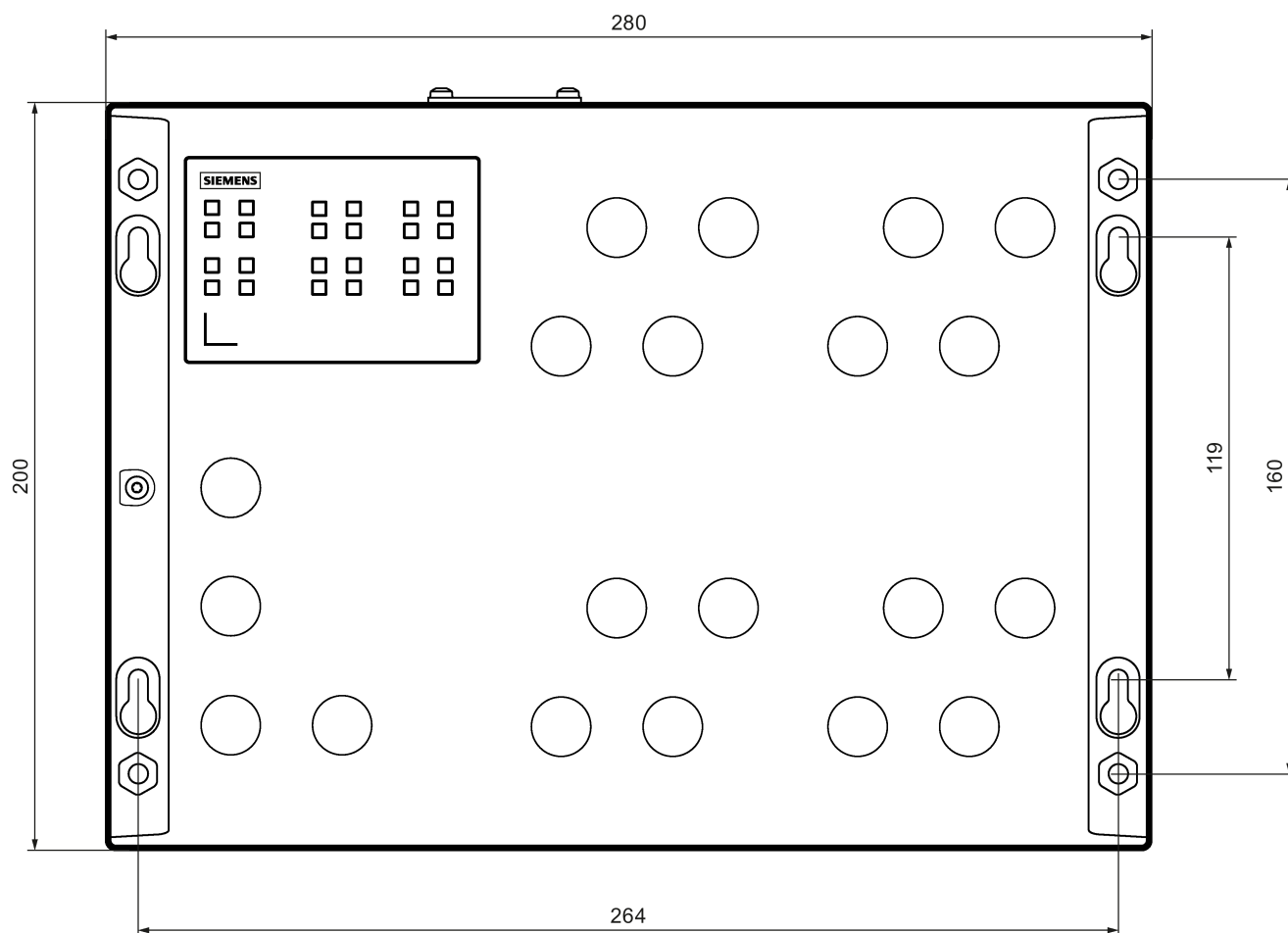
Figure 7-2 Width, height and dimensions for wall mounting
