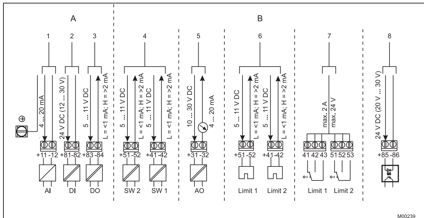
Fig. 8: Pin configuration
