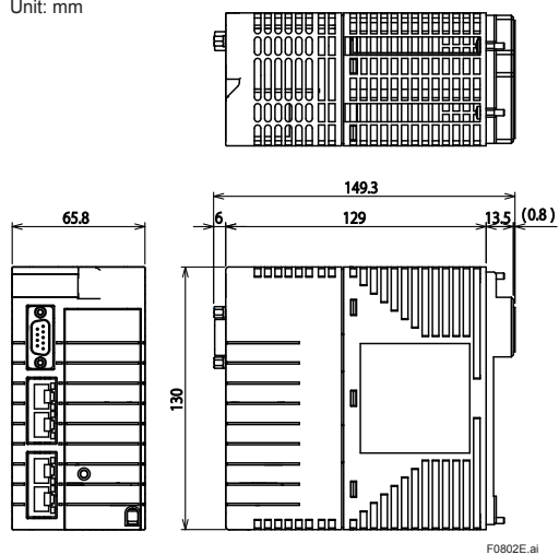
Figure NCP502 (Dimension)
