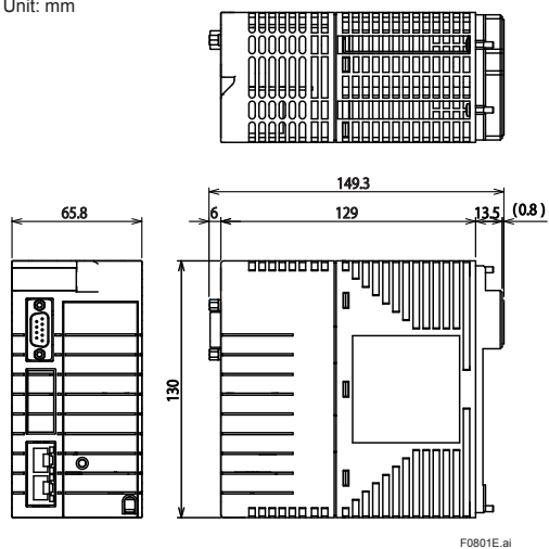
Figure NCP501 (Dimension)
