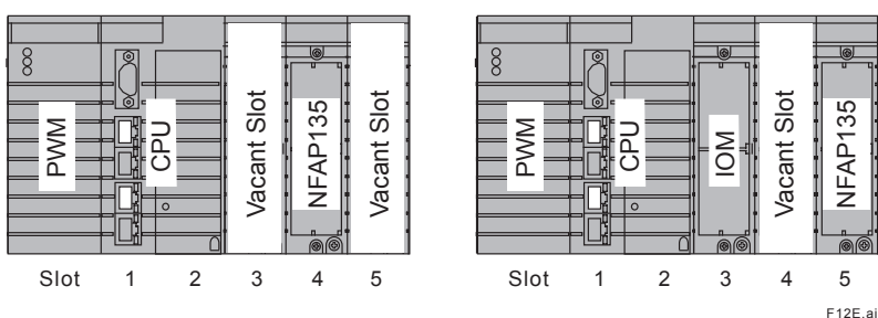
Figure Installation Example of using NFAP135
