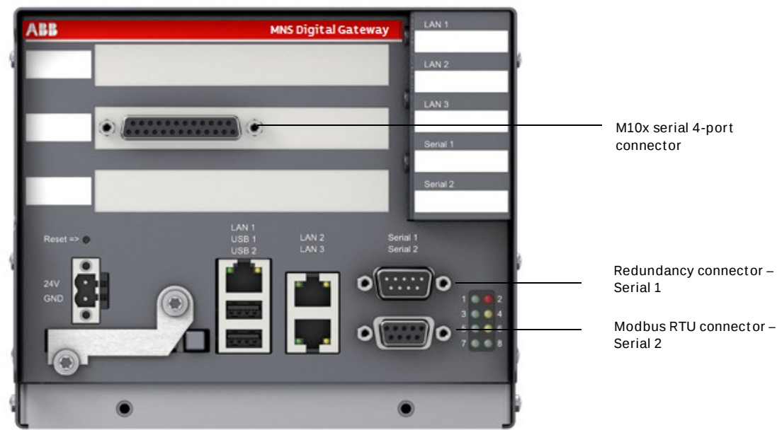
Figure 4 MNS Digital Gateway front view
