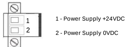
Figure 5 Power Supply Connector
