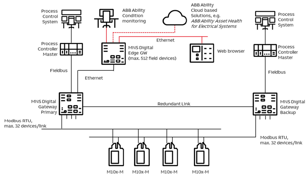
Figure 21 Redundancy configuration and possible failure scenario
