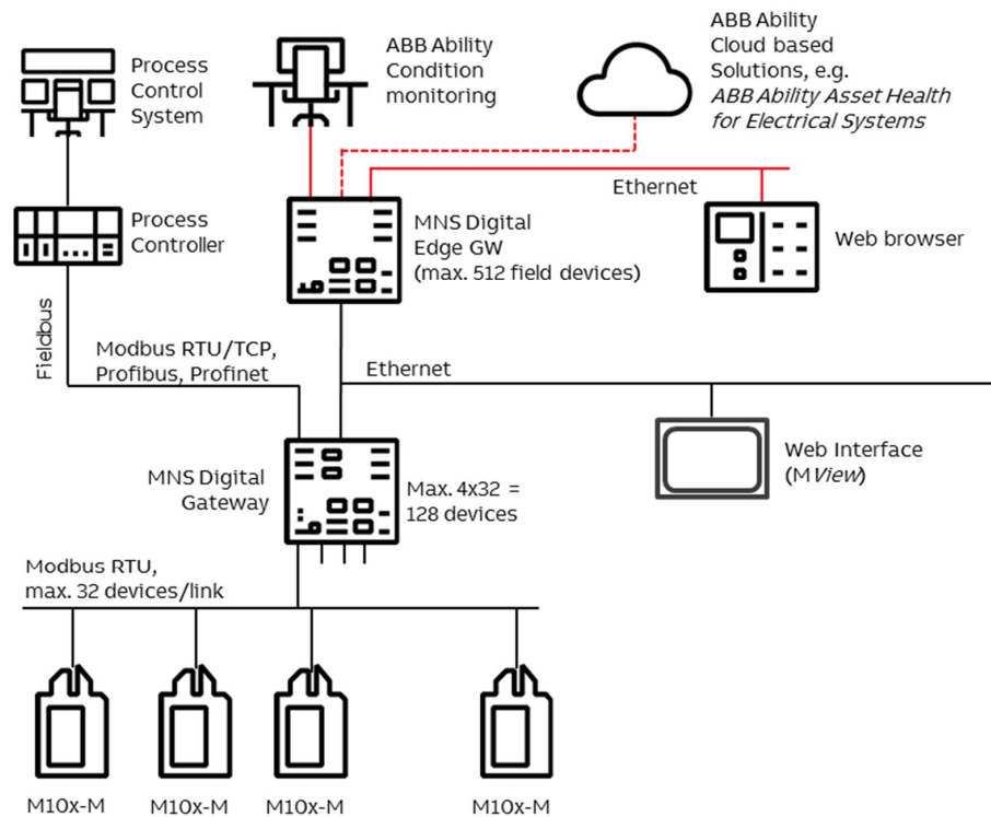
Figure 2: MNS Digital System Configuration with M10x
