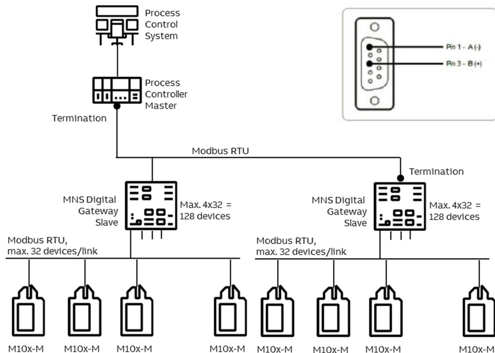
Figure 17 MNS Digital Gateway RS485 connection via Serial 2
