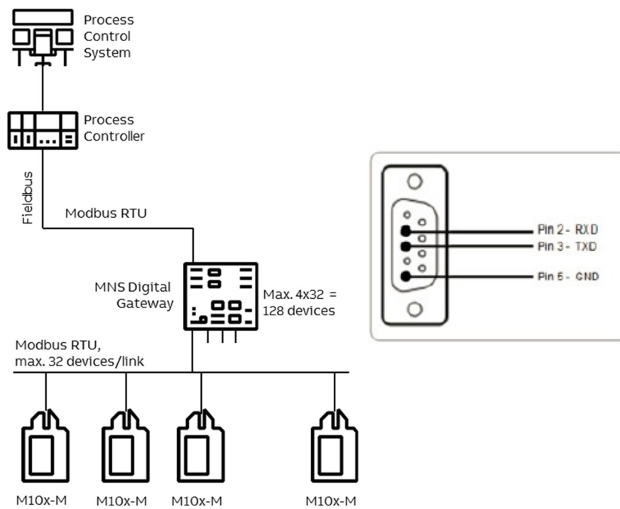
Figure 15 MNS Digital Gateway RS232 connection via Serial 2
