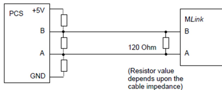
Figure 18 Example for RS485 bus termination and biasing:
