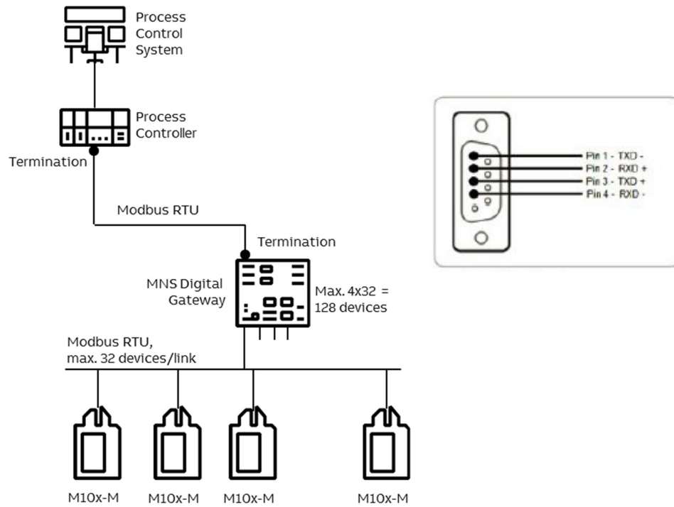
Figure 16 MNS Digital Gateway RS422 connection via Serial 2
