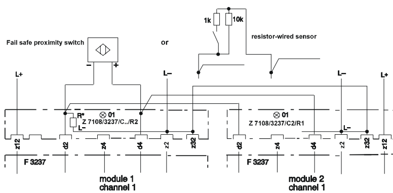
Redundant connection for one proximity switch circuit
