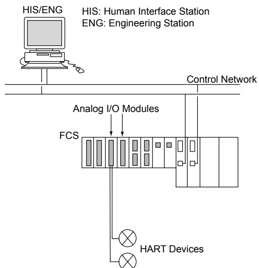
Figure HART Communication System Configuration (Dual-redundant)
