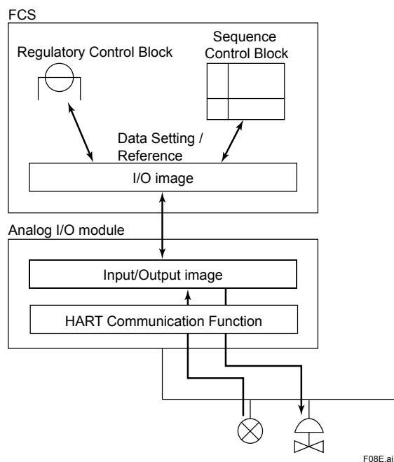
Figure Process Data Flow of HART Communications
