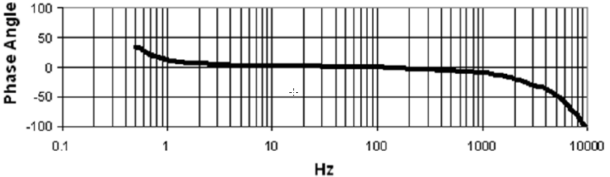
Figure 3 - 4: 200350 Accelerometer Phase
