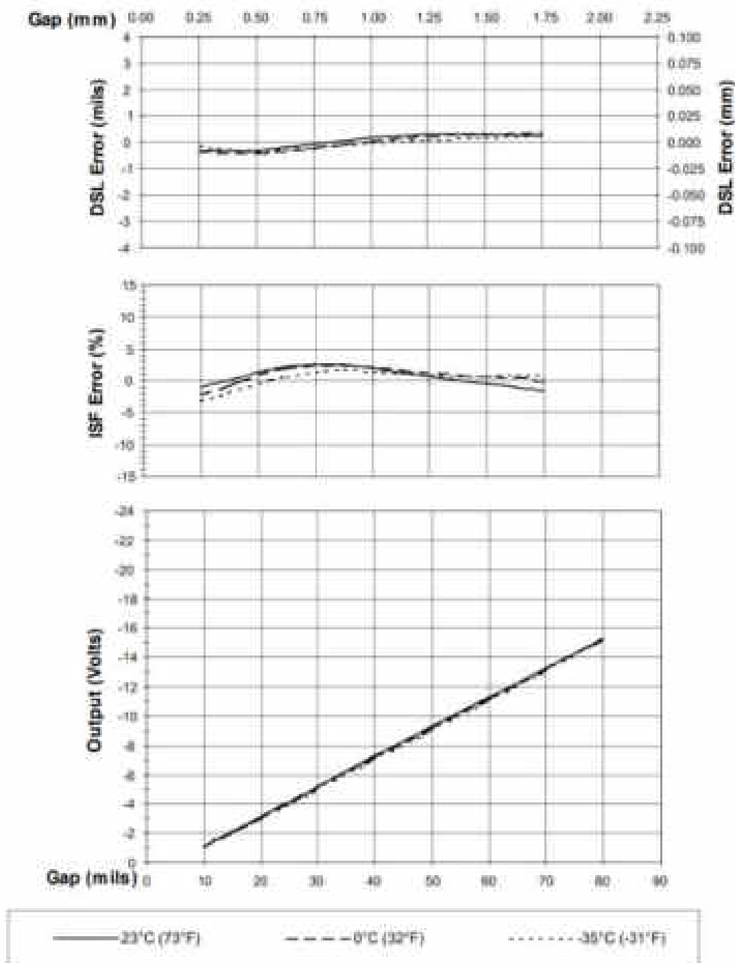
Figure 5: Typical 3300 XL N5v 5 m Proximity Sensor with 4 m of Extension Cable @ Low Temperature (Probe is at 25°C)
