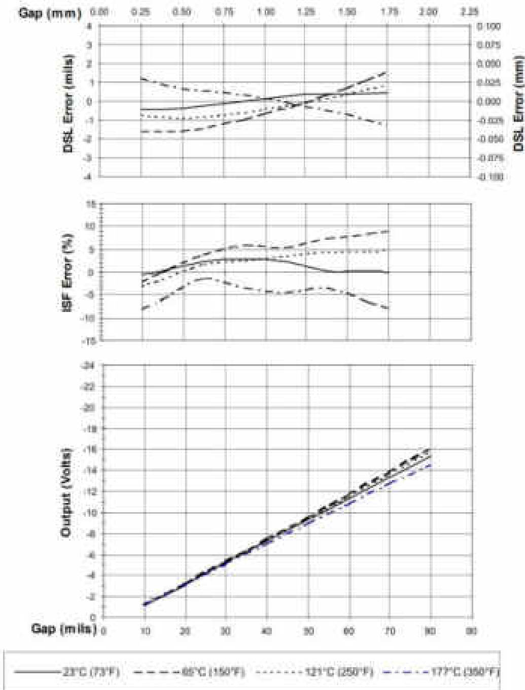
Figure 4: Typical 3200 NSv Probe + 1 m Cable @ High Temperature (Proximity Sensor + 4 m of Extension Cable @ 25°C)
