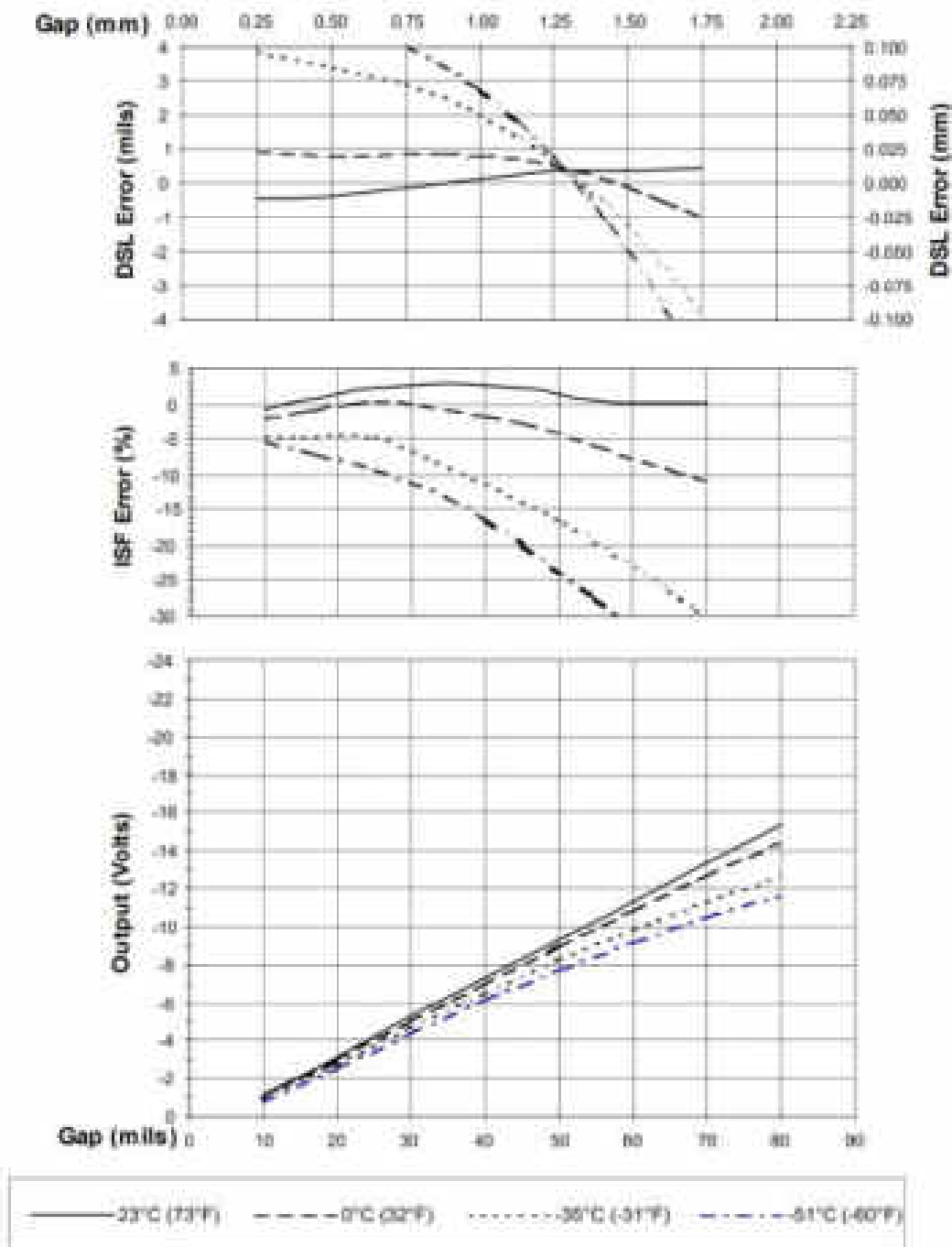
Figure 3: Typical 3200 NSv Probe + 1m Cable @ Low Temperature (Proximity Sensor + 4 m of Extension Cable @ 25°C)
