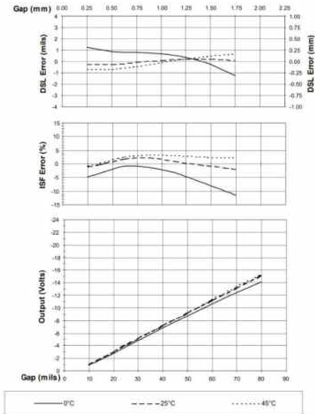
Figure 1: Typical 3200 XL NSv 5 m System over Ambient Temperature Range
