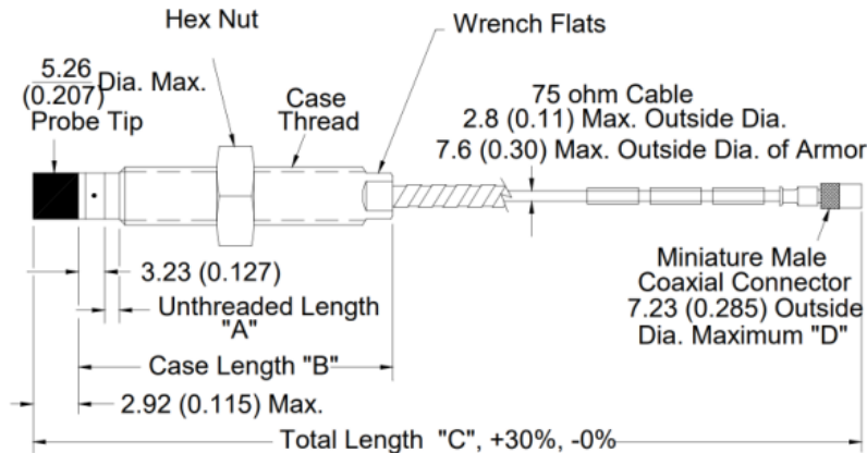
Figure 18: 3300 NSv Proximity probes, Standard Mount
