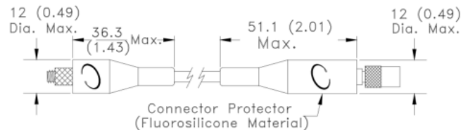
Figure 19: Installed Connector Protectors
