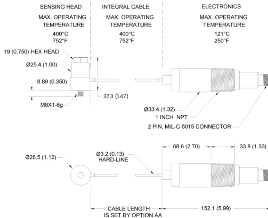
Figure 2: 330752 System Dimensional Drawing
