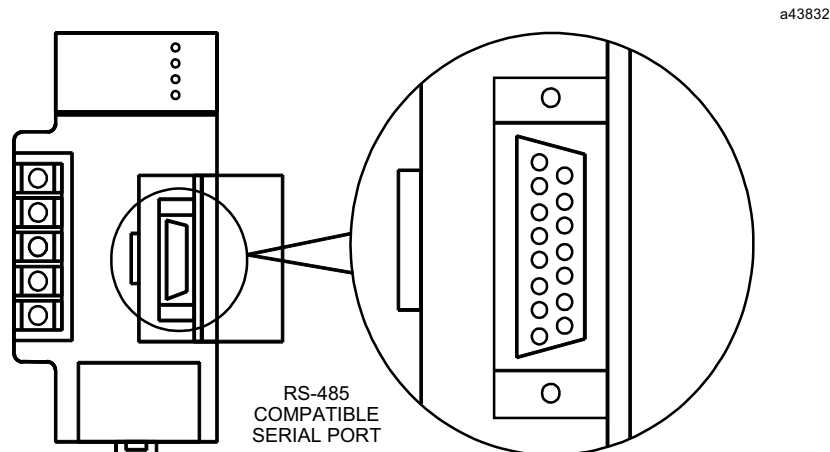
Figure 4-13. Serial Port Connector
