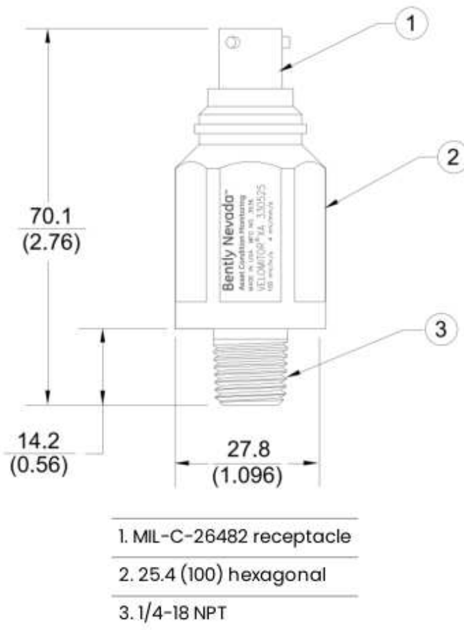
Figure 2: Dimensions for 330525 Velomitor XA Piezo-Sensor Dimensions are in millimeters (inches)
