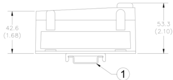
Figure 1: 990 Vibration Transmitter Dimensions (top view)
