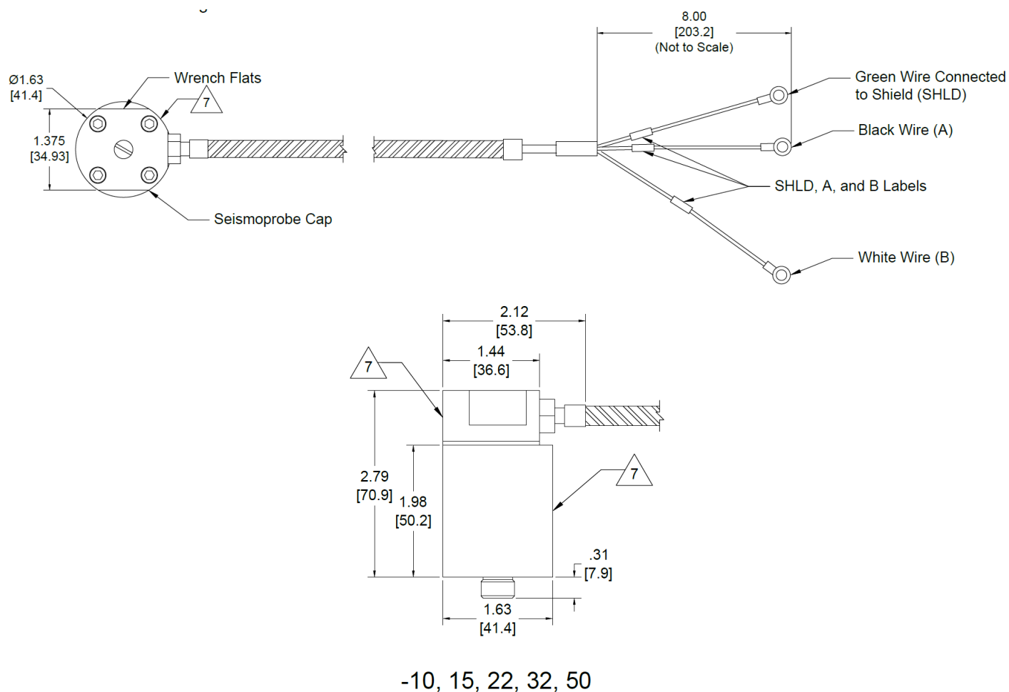
Figure 7: 9200 Standard Integral Cable Options B-10 through B-50
