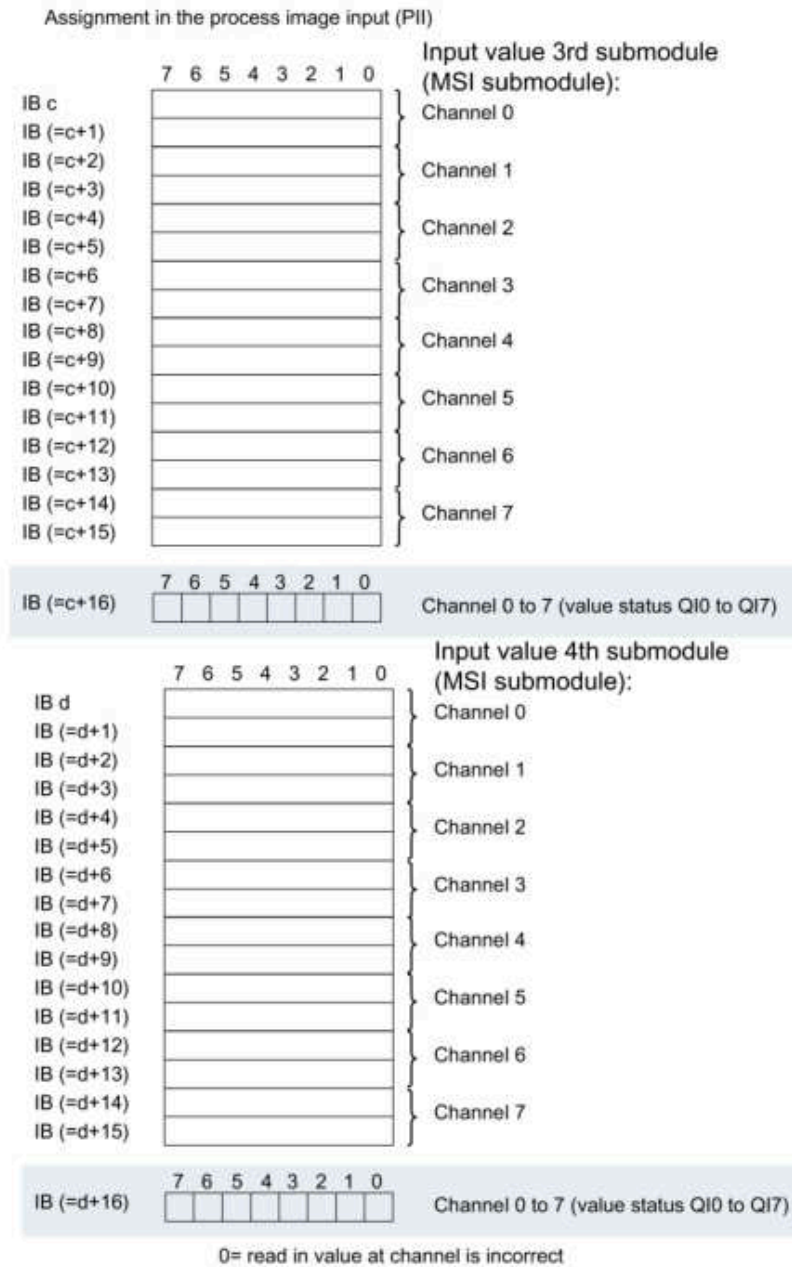
Figure 4-7 Address space for configuration as 1 x 8-channel AI 8xU/I/RTD/TC ST MSI with value status
