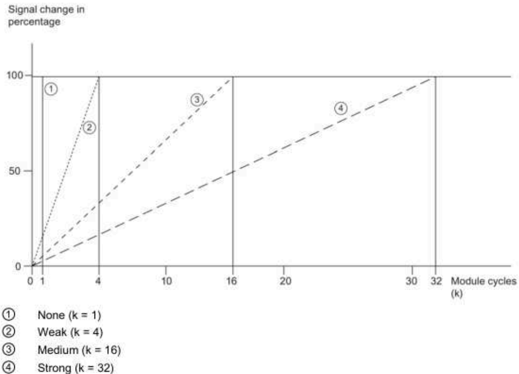
Figure 4-3 Smoothing with AI 8xU/I/RTD/TC ST
