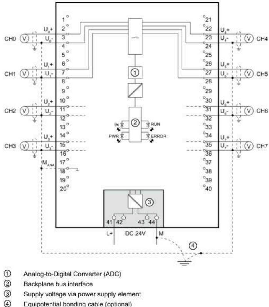
Figure 3-2 Block diagram and pin assignment for voltage measurement
