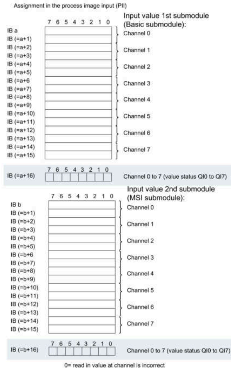
Figure 4-6 Address space for configuration as 1 x 8-channel AI 8xU/I/RTD/TC ST MSI with value status
