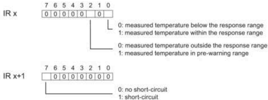
Figure 4-1 Address space for AI 8xU/I/RTD/TC ST with PTC resistors
